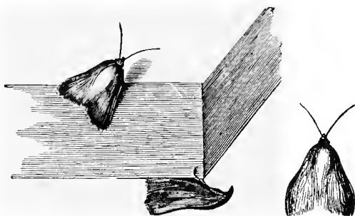
Fig. 89.—BEE MOTH.
